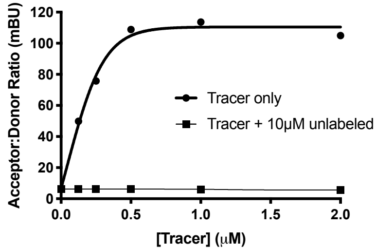
NL-HIPK4 tracer 10-7600 CTx-0294885 EC50
