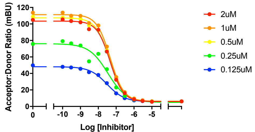
NL-HIPK4 tracer 10-7600 CTx-0294885
